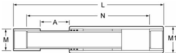
1-1/4" & Up Configuration
