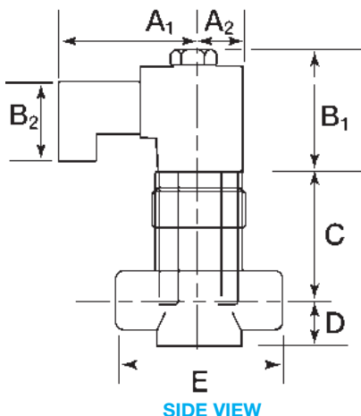
SOLENOID VALVE BODY DIMENSIONS
