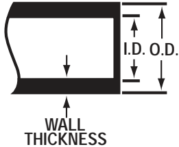
SCHEDULE 40 PIPE DIMENSIONS ASTM D 1785
