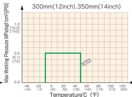
Gate Valve TypeP, Type S
